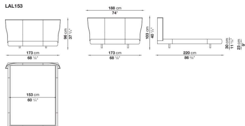
LAL153
