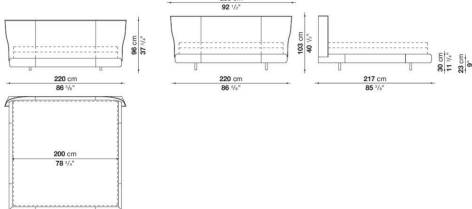
LAL200
